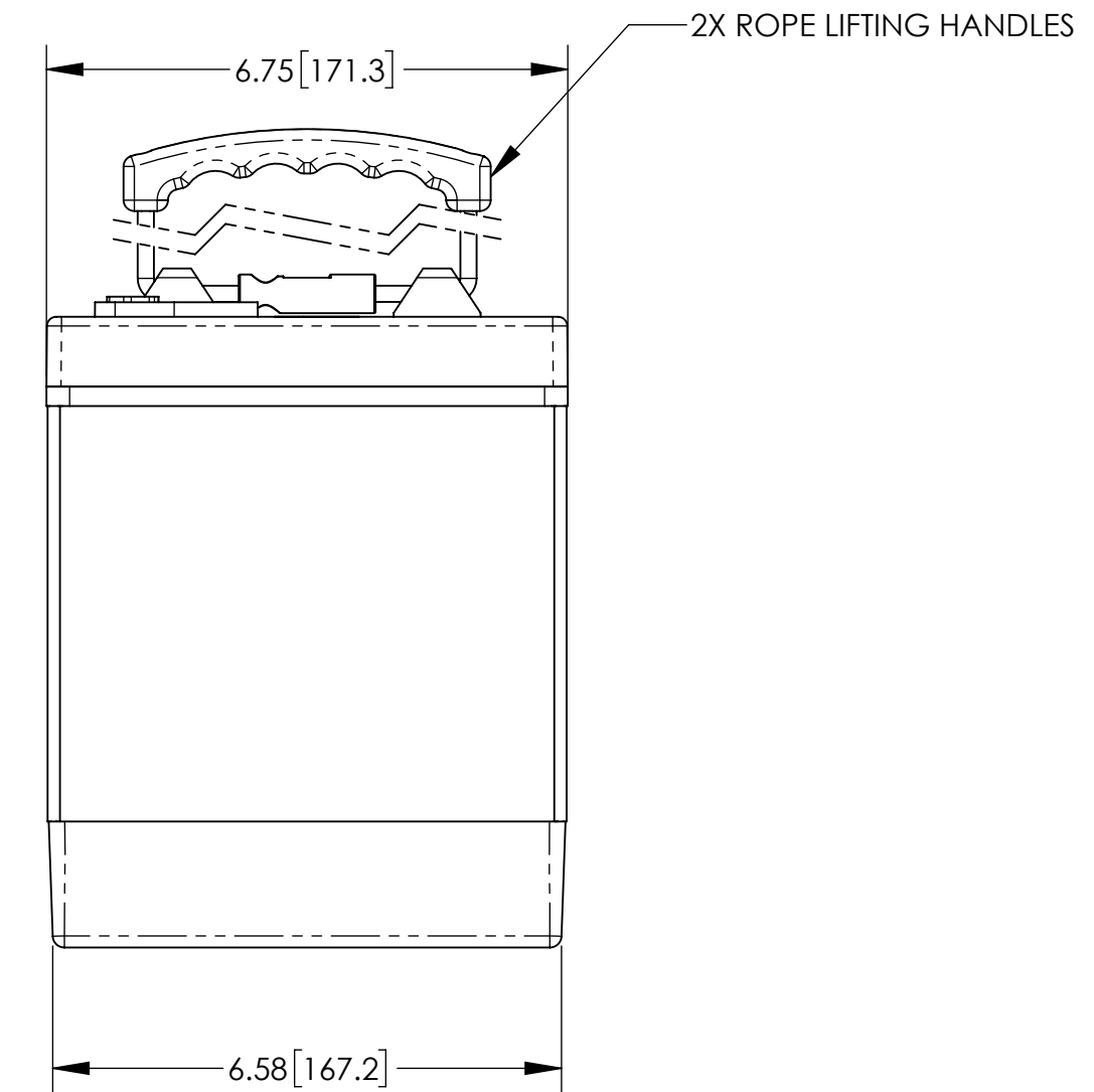
ENVELOPE DRAWING
