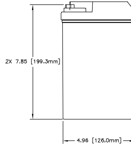
ENVELOPE DRAWING
